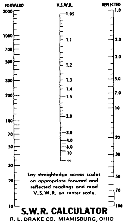
Figure 3-3. SWR Nomograph
