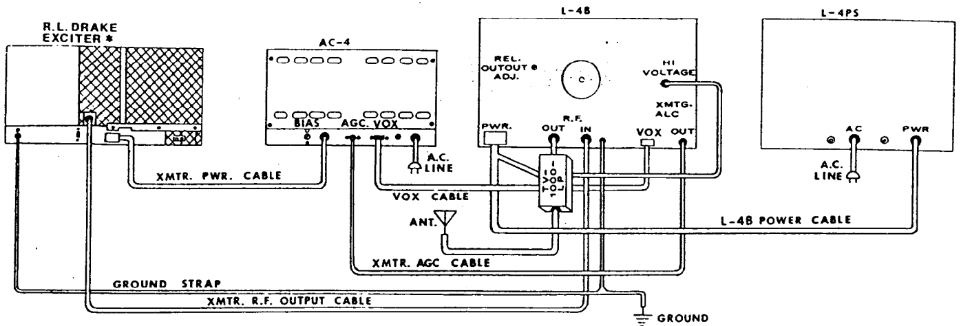
Figure 2-4. Connecting the AC-4 Power Supply and the R. L. Drake Line of Compatible Exciters.
