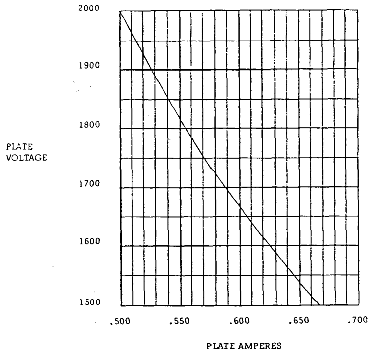
Figure 3-2. Plate Voltage and Plate Current VS 1,000 Watts DC Input Power
