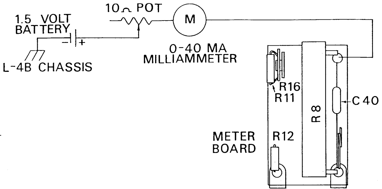
Figure 5-3. Connections for Grid Current Meter Calibration
