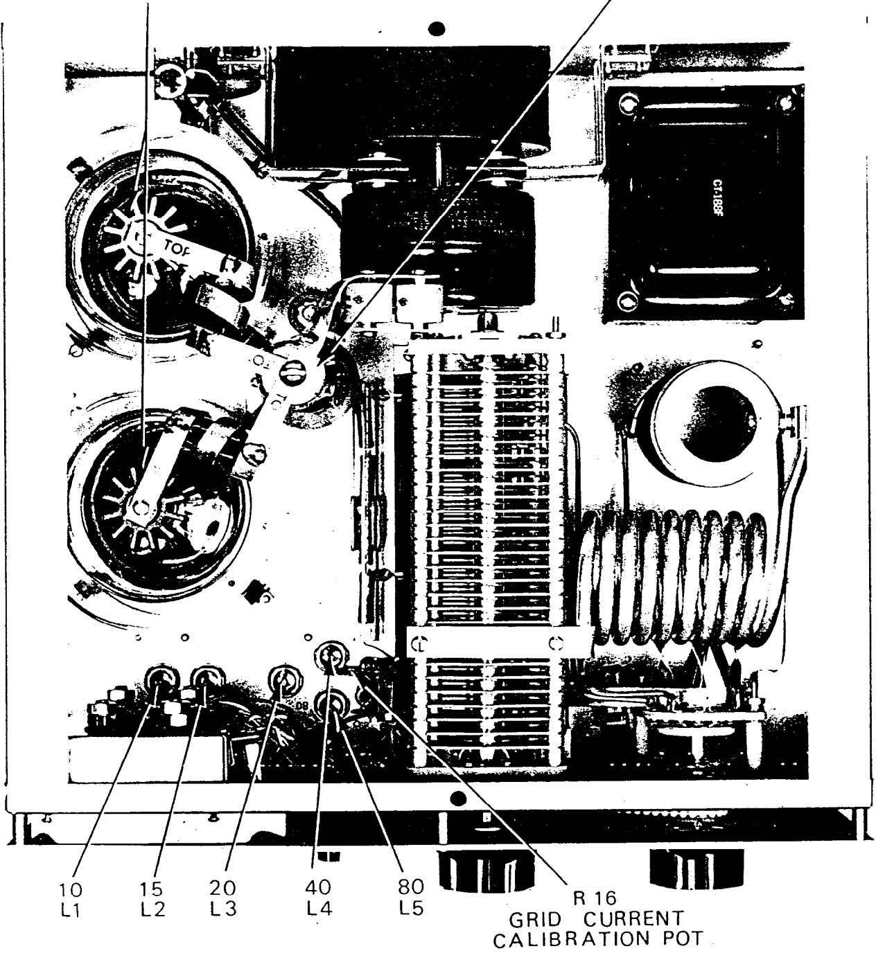
Figure 5-1. Component Locations, Top View
