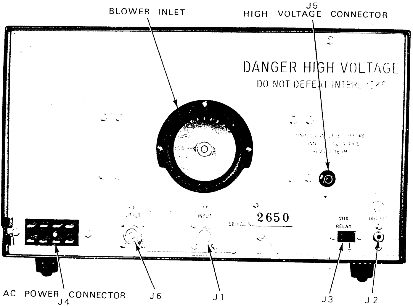
Figure 2-1. Rear Chassis Connectors
